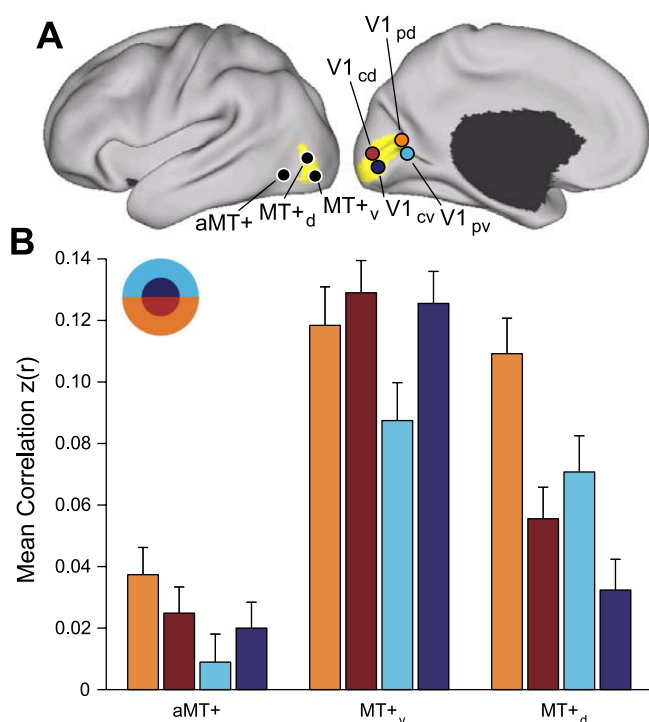
Fig. 22. Functional connectivity between MT+ and V1 is topographically organized. A : 2 MT+ seed regions, MT d and MT v , were selected in the dorsal and ventral portions of the histological MT+ estimate, respectively. The anterior MT+ (aMT+) seed region was selected anterior to histological MT+. Four V1 seed regions were selected using the histological V1 estimate: V1 cd and V1 cv were selected in dorsal and ventral central V1; V1 pd and V1 pv were selected in dorsal and ventral peripheral V1. Coordinate locations of seed regions are reported in Table 2. B : correlation strength of aMT+ and MT+ seed regions with V1 in the replication dataset. There are 4 observations to be noted: 1) V1-aMT+ correlation is weaker than V1-MT+ correlation, 2) MT+ correlation with the lower visual field is stronger than the upper visual field, 3) MT d correlation with peripheral V1 is stronger than central V1, and 4) MT v correlation with central V1 is stronger than peripheral V1.
